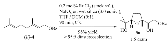
Scheme 3. Gram scale oxidative cyclization of geranyl benzoate [( E )-4] under optimized conditions.
