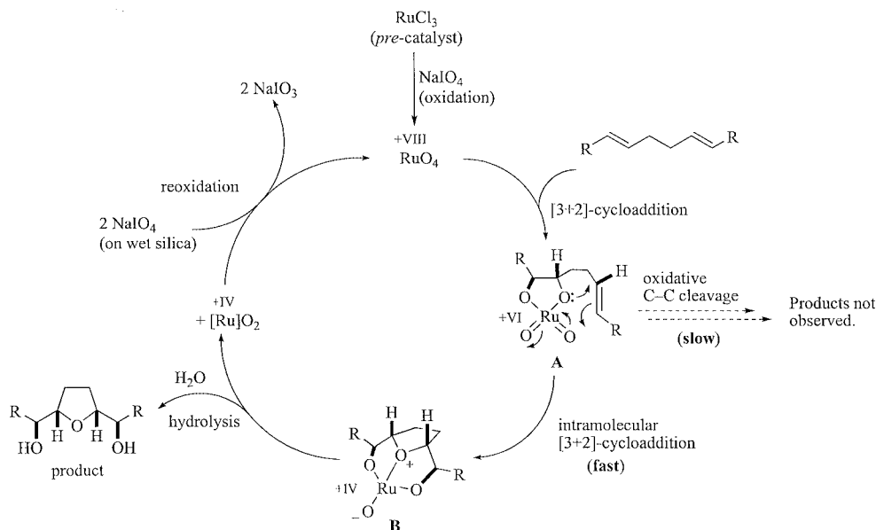
Scheme 5. Proposed mechanism for the ruthenium tetroxide catalyzed oxidative cyclization of 1,5-dienes.
