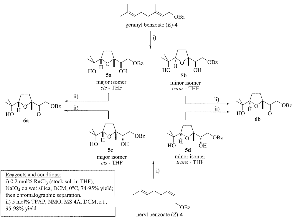
Scheme 4. Stereochemical correlation of oxidative cyclization products.
